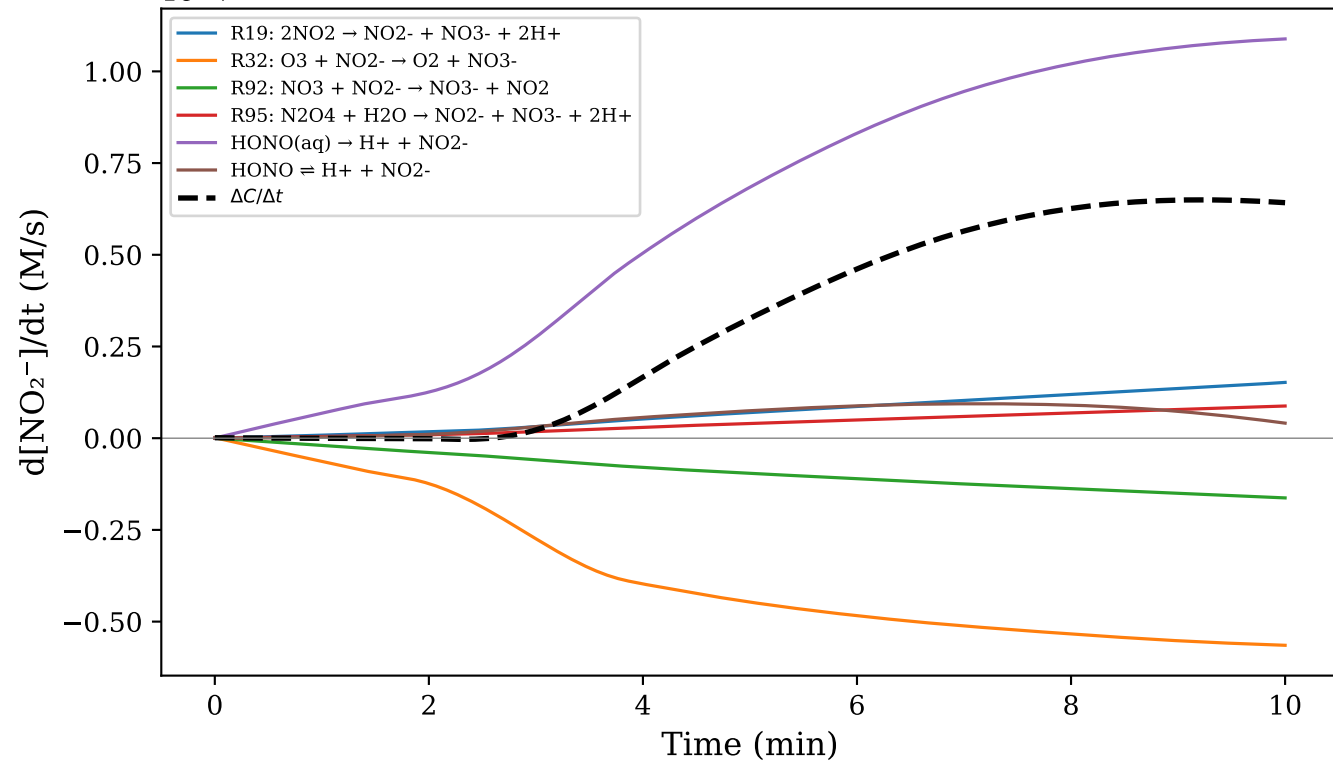
(c) \text{NO}_2^-
